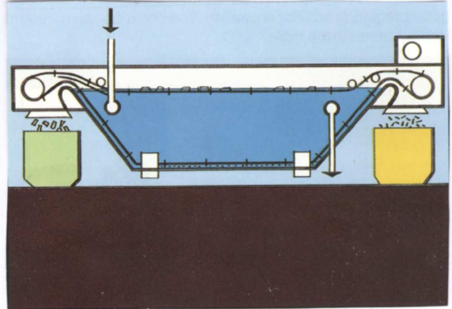
This cleaning basin - available in all sizes - has plastic chains and pushers to remove submerged particles as well as particles floating on the surface. The two types of particles are removed on opposite sides.
