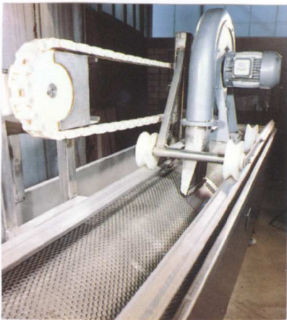
The cleaning device of our separator has its own air supply.
