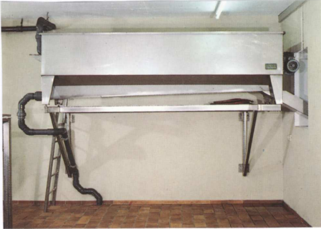
Separator with automatic cleaning device. Available in two different sizes, also without cleaning device.
